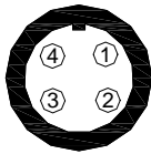
4 pins Binder 712 female connector front view
