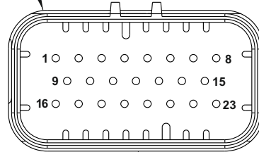
23 PIN AMP PANEL MALE CONNECTOR PINOUT EXT VIEW
